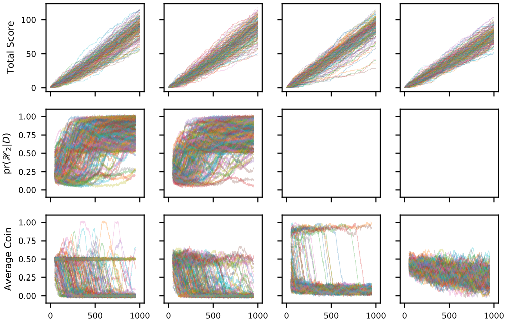
Bayes
